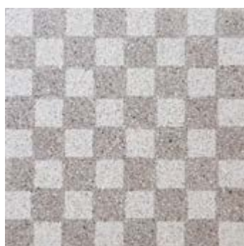
GRANIT BEIRÃO MDJ4020811 GRANITO BEIRÃO 60x60x2,5 cm ≈ 62 Kg/m 2
